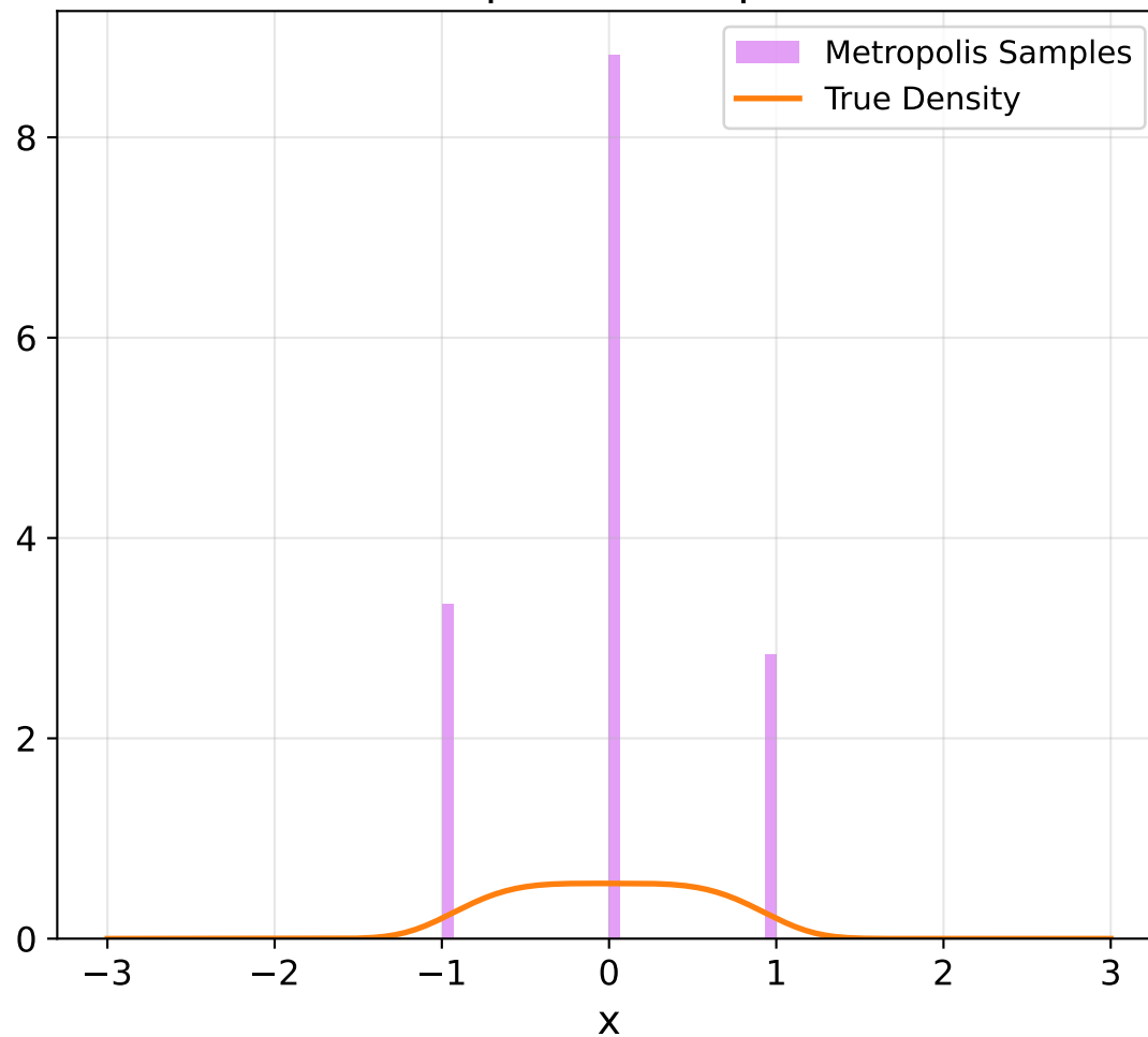
Random Walk (Step=1), Acceptance Rate=0.42
