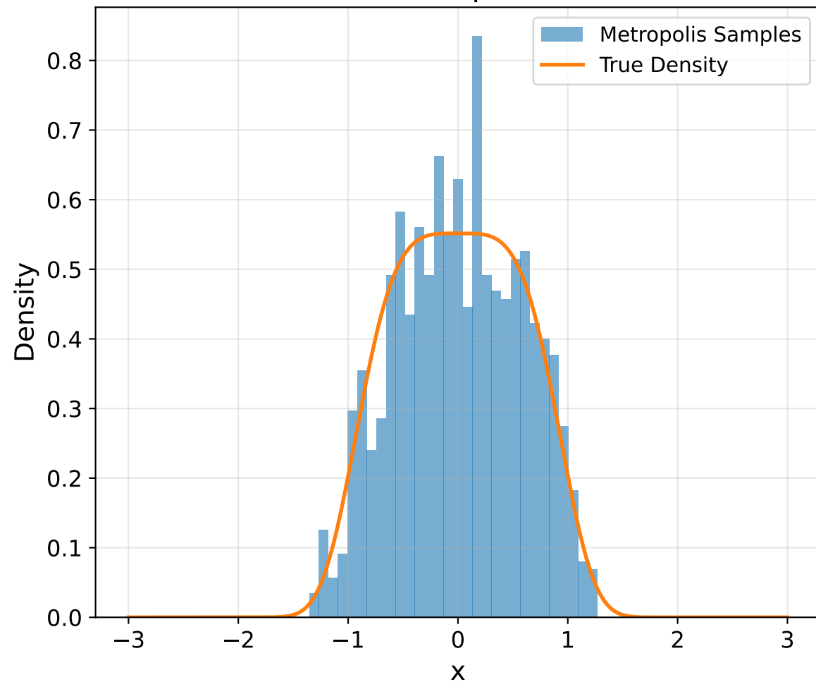
Uniform(-1, 1), Acceptance Rate=0.72
